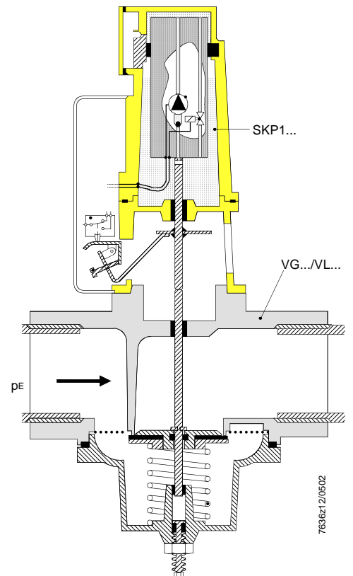
Sectional view VGG... complete with SKP1...
