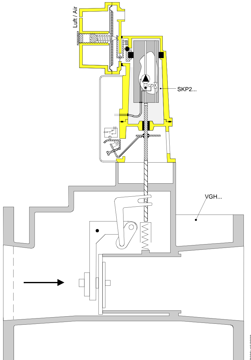
Sectional view VGH... complete with SKP2...
